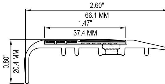
ECOGLO-PROFILE C5 SERIES WITH E20 SERIES INSERT
